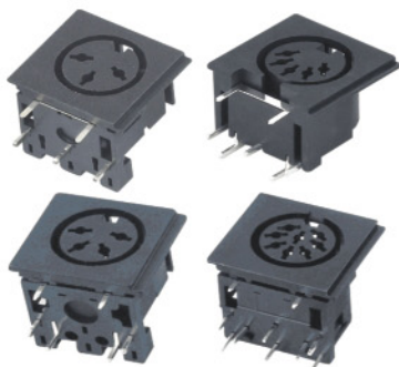
21001-XXP-700 XX:03P~08P,13P (大DIN)
