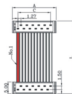
Double End-C Type
