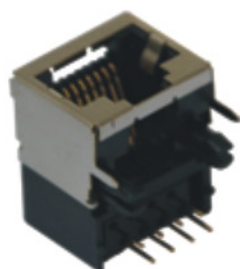
22003-5321S-8P8C
