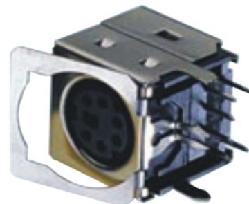
21005-5M-XXP XX:03P~08P(帶彈片MINI DIN)
