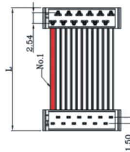
Single End-H Type
