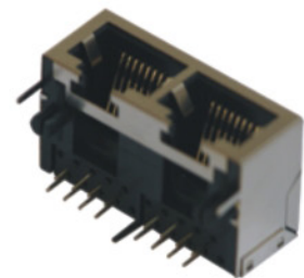
22003-5622S-10P8C*2脚前
