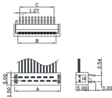
Single End-G Type
