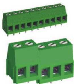
MB310-500/505/750M
