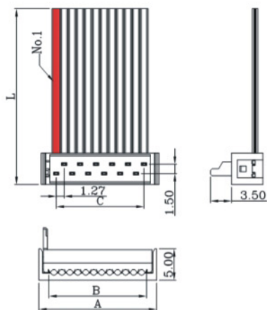
Single End-B Type
