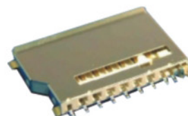
SDCMF-209XXW0T0 Secure Digital Card Short Type
